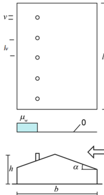
Figure 5.7.a NA Closely spaced local shelters with wind from easterly directions, cf. Figure 5.2.c NA
